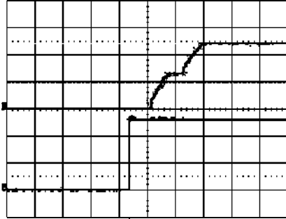
Start-up enabled by connecting V_i at: T_{ref} = +25^\circ\text{C} , I_o = 10.5\text{ A} resistive load, V_i = 53\text{ V} . Top trace: output voltage (5 V/div). Bottom trace: input voltage (20 V/div). Time scale: 10ms/div.
