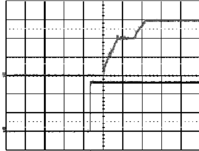
Start-up enabled by connecting V_i at: T_{ref} = +25^{\circ}\text{C} , I_o = 30\text{ A} resistive load, V_i = 53\text{ V} . Top trace: output voltage (0.5 V/div). Bottom trace: input voltage (20 V/div). Time scale: (10ms/div).
