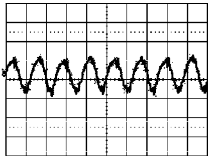
Output voltage ripple (50mV/div) at: T_{ref} = +25^{\circ}\text{C} , I_O = 35\text{ A} resistive load, V_i = 53\text{ V} . Time scale: 2 \mu\text{s} /div See the filter in the Output ripple and noise section (EMC Specification).
