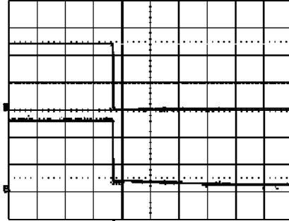
Shut-down enabled by disconnecting V_i at: T_{ref} = +25^\circ\text{C} , I_o = 10.5\text{ A} resistive load, V_i = 53\text{ V} . Top trace: output voltage (5 V/div). Bottom trace: input voltage (20 V/div). Time scale: 5 ms/div.
