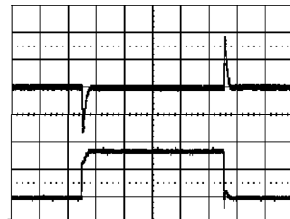
Output voltage response to load current step- Top trace: output voltage (100mV/div). change (8.75-26.25-8.75 A) at: T_{ref} = +25^{\circ}\text{C} , V_i = 53\text{ V} . Time scale: 0.1 ms/div.
