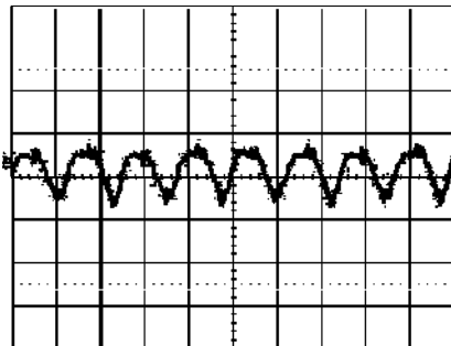
Output voltage ripple (50mV/div) at: T_{ref} = +25^\circ\text{C} , I_o = 15\text{ A} resistive load, V_i = 53\text{ V} . Time scale: 2 \mu\text{s} /div. See the filter in the Output ripple and noise section (EMC Specification).
