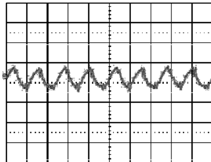
Output voltage ripple (50mV/div) at: T_{ref} = +25^{\circ}\text{C} , I_o = 30\text{ A} resistive load, V_i = 53\text{ V} . Time scale: 2 µs/div See the filter in the Output ripple and noise section (EMC Specification).
