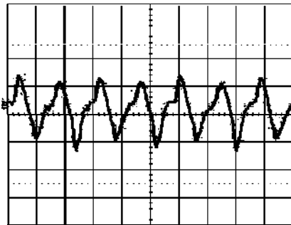
Output voltage ripple (50mV/div) at: T_{ref} = +25^\circ\text{C} , I_o = 10.5\text{ A} resistive load, V_i = 53\text{ V} . Time scale: 2 \mu\text{s} /div See the filter in the Output ripple and noise section (EMC Specification).
